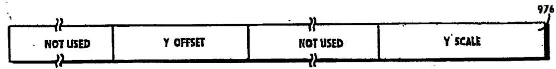
Fig. 35N VIDEO INTERFACE Y SCALE REGISTER (R/W)
